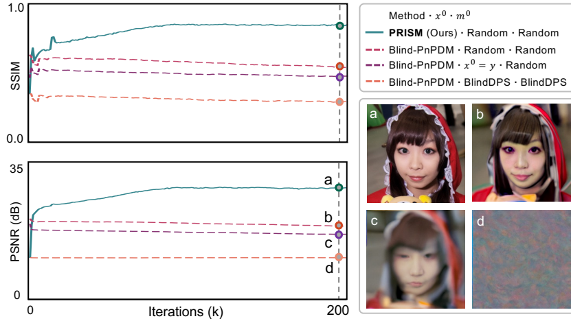
Figure 2: Convergence comparison between PRISM and Blind-PnPDM [14]. Results for Blind-PnPDM are shown for three different initialization settings. Note that Blind-PnPDM struggles to converge to a reasonable image with fully random initializations, while PRISM achieves steady convergence to a high-quality image.
